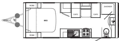
RANGE: MANTA RAY MODEL: MR18ES3
