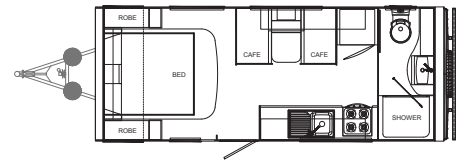
RANGE: MANTA RAY MODEL: MR18ES4
