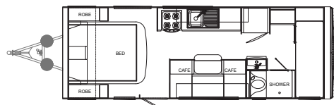
RANGE: MANTA RAY MODEL: MR20ES2
