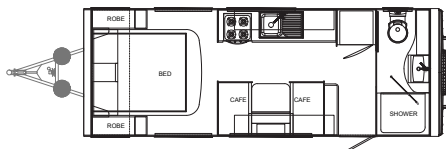
RANGE: MANTA RAY MODEL: MR19ES2 (CAFE)
