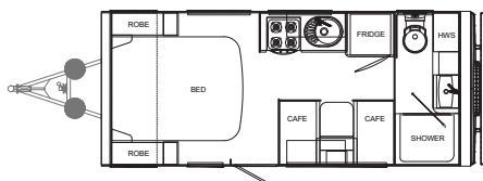
RANGE: MANTA RAY MODEL: MR16ES3
