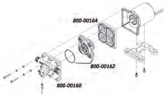
800-00164 REPLACEMENT DRIVE ASSEMBLY #3
